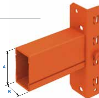
2C-S beam (1115)
