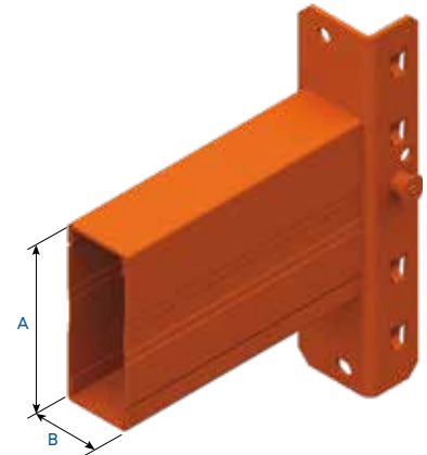
2C-S beam (1315, 1515, 1615, 1718)
